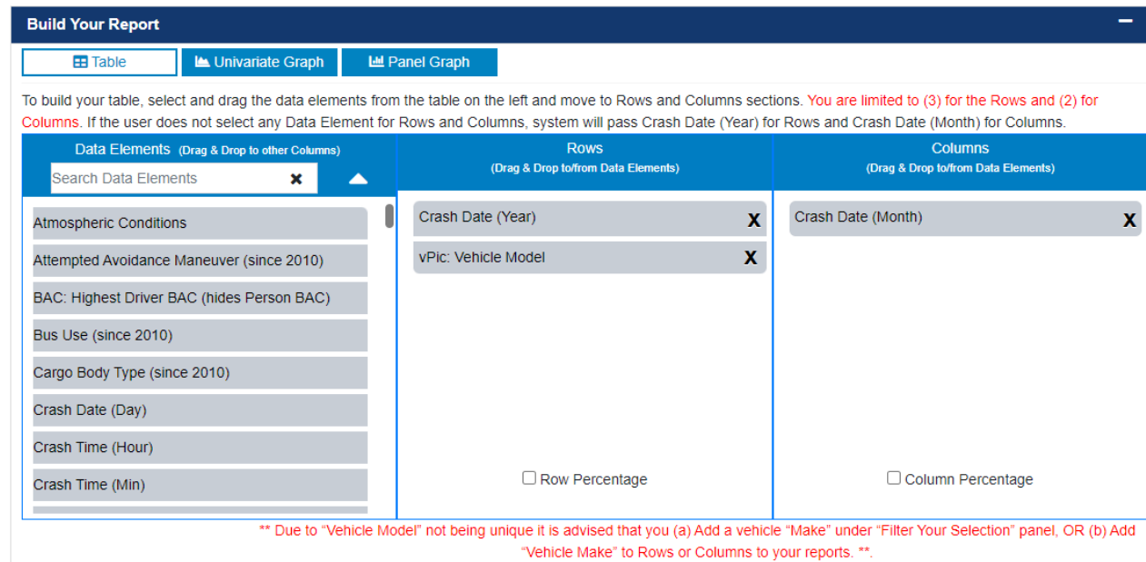
Figure 28 – Message for Using Vehicle Model and Striking Vehicle Model in Build Your Reports
