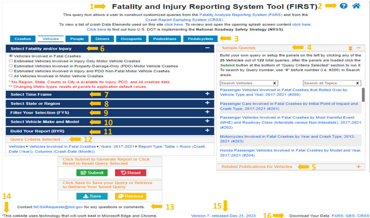
Figure 3 – Screenshot of FIRST Screen Showing Vehicles Topic
